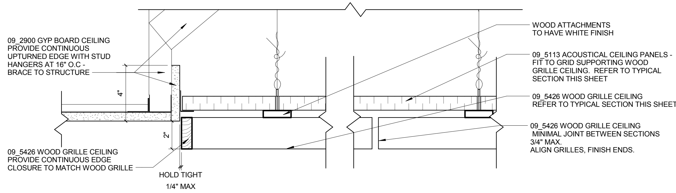
10 WOOD GRILLE CEILING EDGE DETAIL 3\"/>
