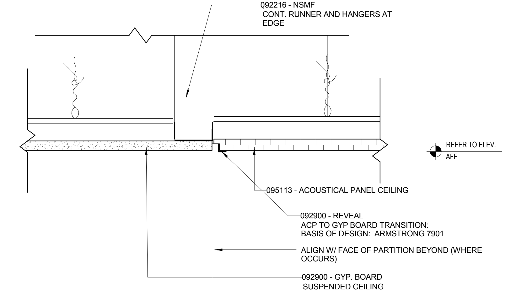
2 GWB TO APC TYP TRANSITION DETAIL 3\"/>
