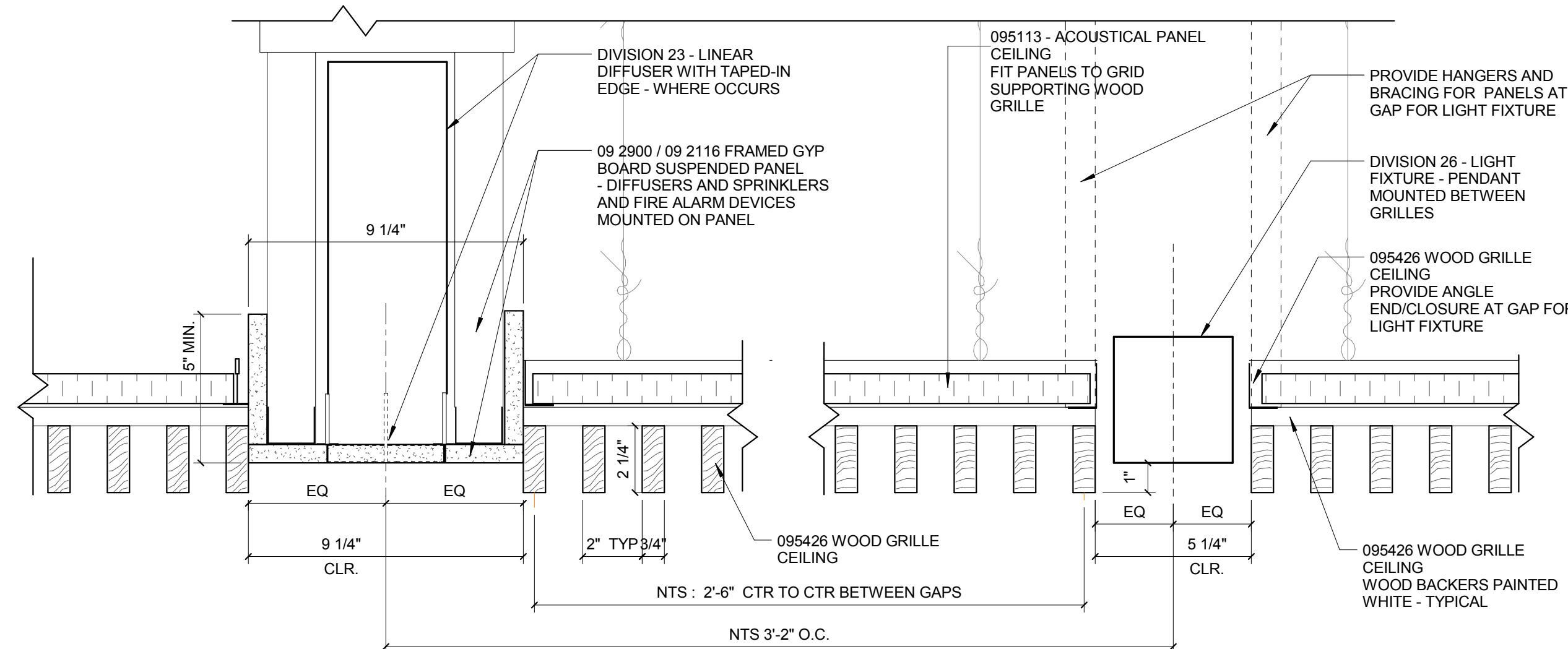
9 WOOD GRILLE CEILING DETAIL 3\"/>
