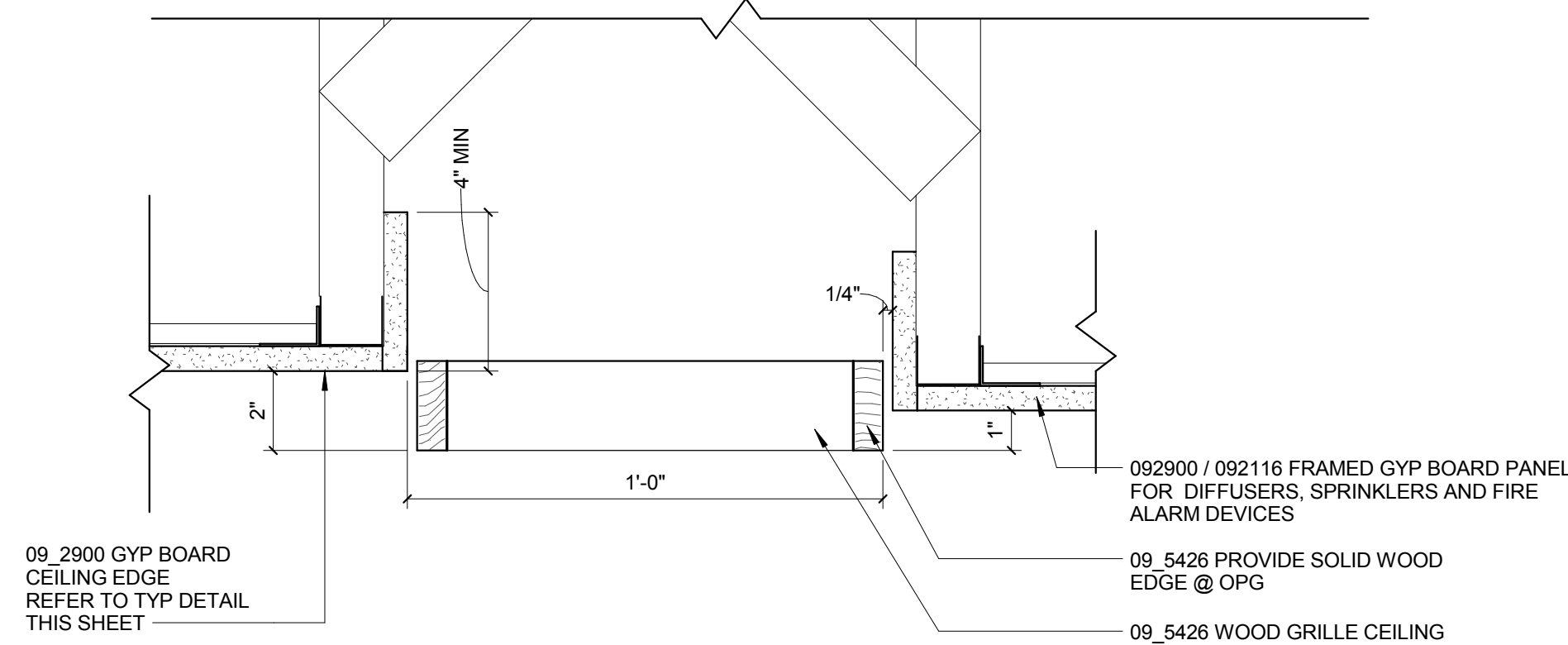
5 A0841 EDGE DETAIL AT DIFFUSER 3\"/>
