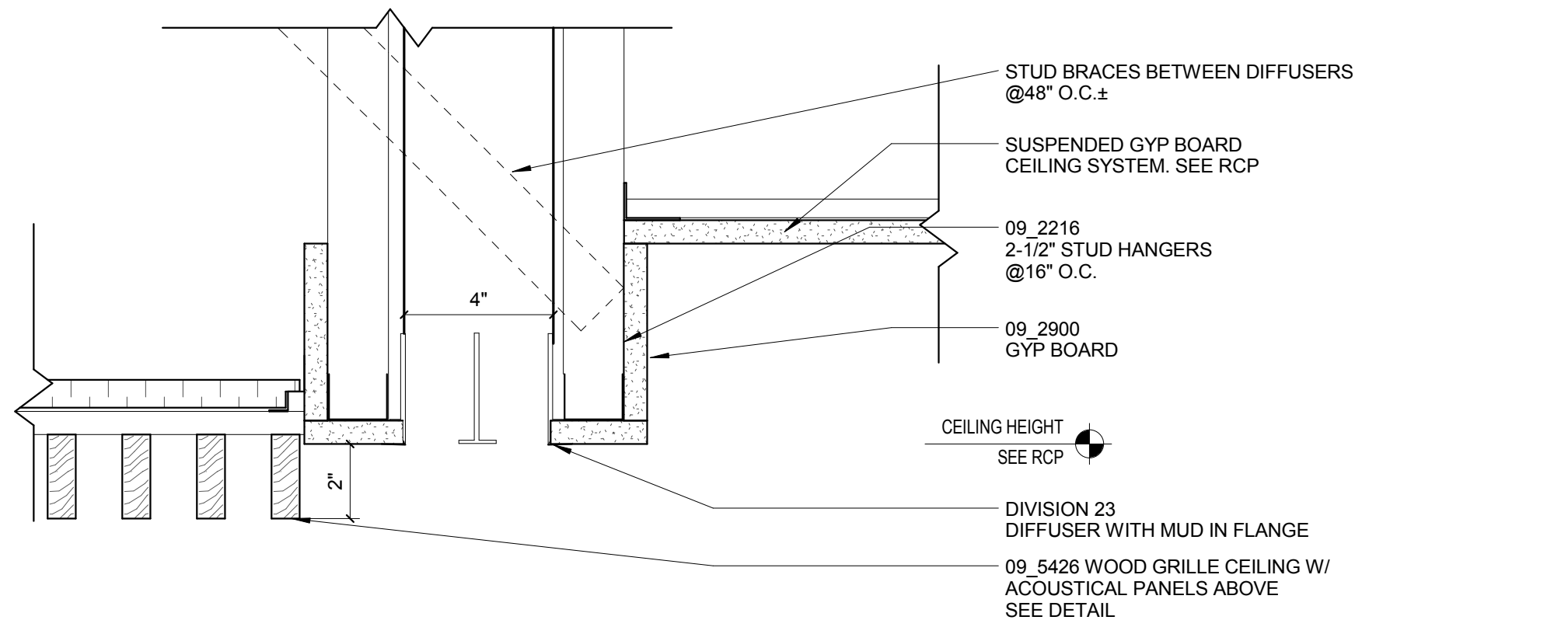
11 A0841 WOOD GRILLE CEILING EDGE DETAIL 3\"/>
