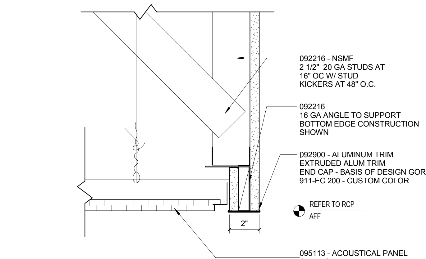
4 ACP EDGE AT OPENING 3\"/>
